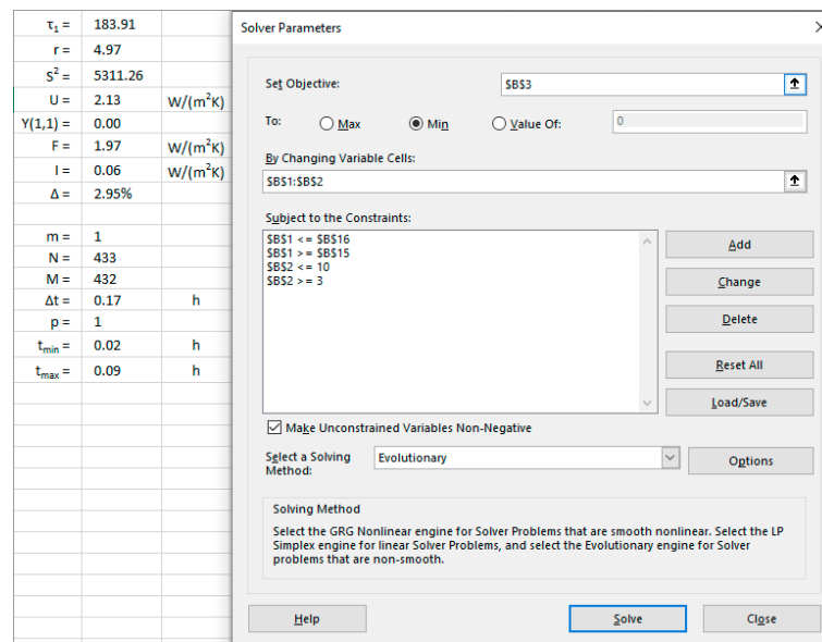
Figure 4. Microsoft Excel Solver parameters for U-value determination.
