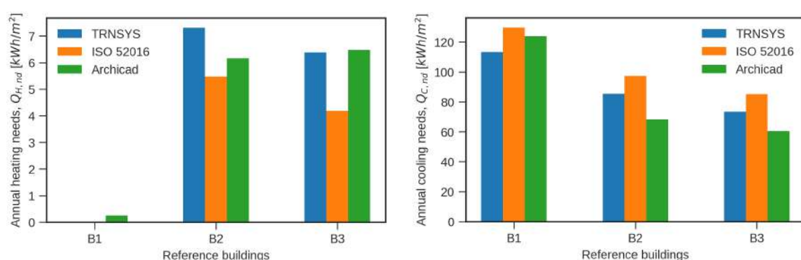
Figure 12. Annual heating and cooling needs for analyzed buildings in littoral climate for three types of energy simulation: TRNSYS (blue), ISO 52016-1:2017 (ISO 52016, orange), and Archicad Energy Evaluation tool (Archicad, green).
