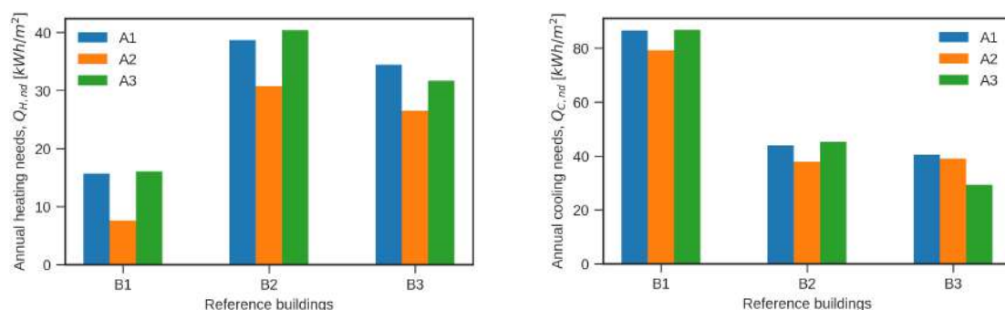
Figure 13. Comparison of the results described in Section 4.2.1—A1 with the results for directly downloaded weather data—A2, and the results for constructions with lower LOD—A3. The results are for continental climate and Energy Evaluation tool.
