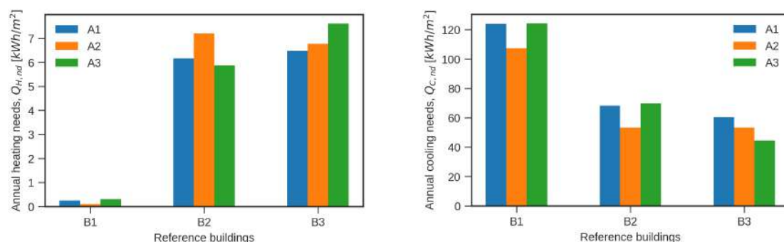
Figure 14. Comparison of the results described in Section 4.2.1—A1 with the results for directly downloaded weather data—A2, and the results for constructions with lower LOD—A3. The results are for littoral climate and Energy Evaluation tool.
