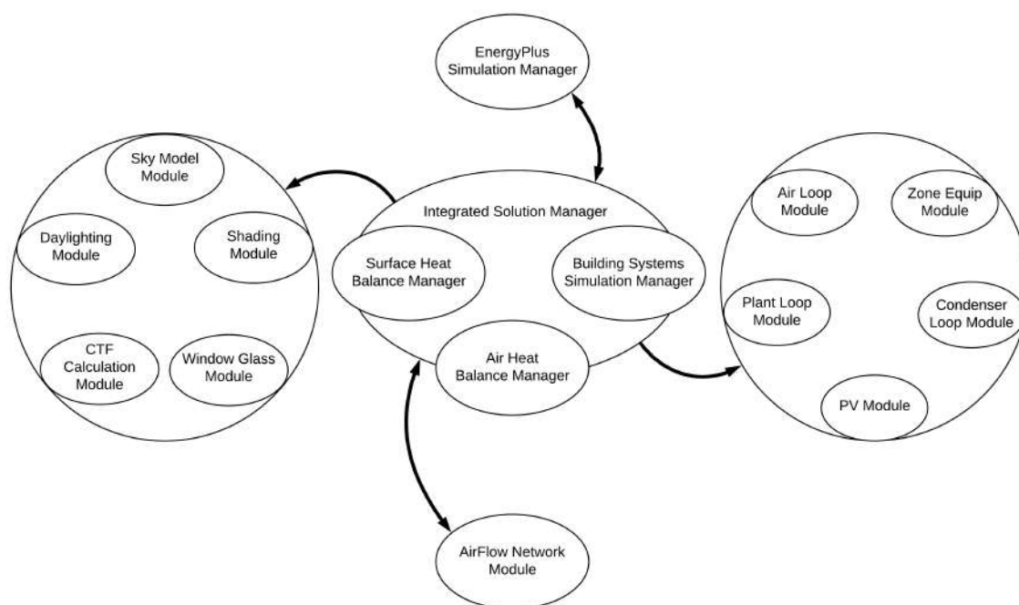
Figure 3. Example of schematic description of commonly used software for dynamic simulation of building energy (EnergyPlus).
