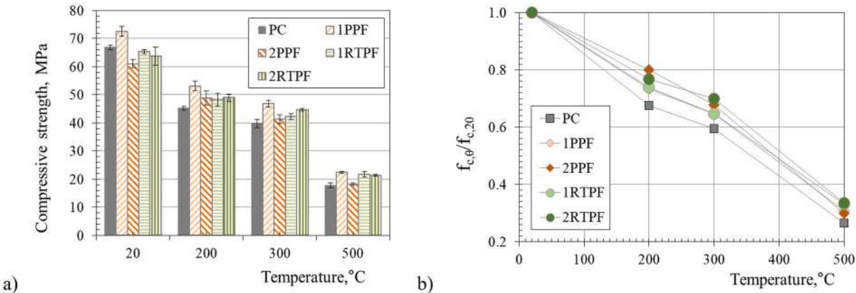
Fig. 10. Residual compressive strength vs temperature: a) mean and b) relative values.
