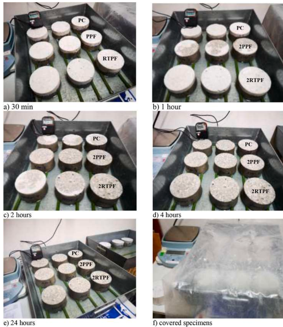
Fig. 13. Specimens heated to 500 °C for capillary absorption test at different time frames of testing.
