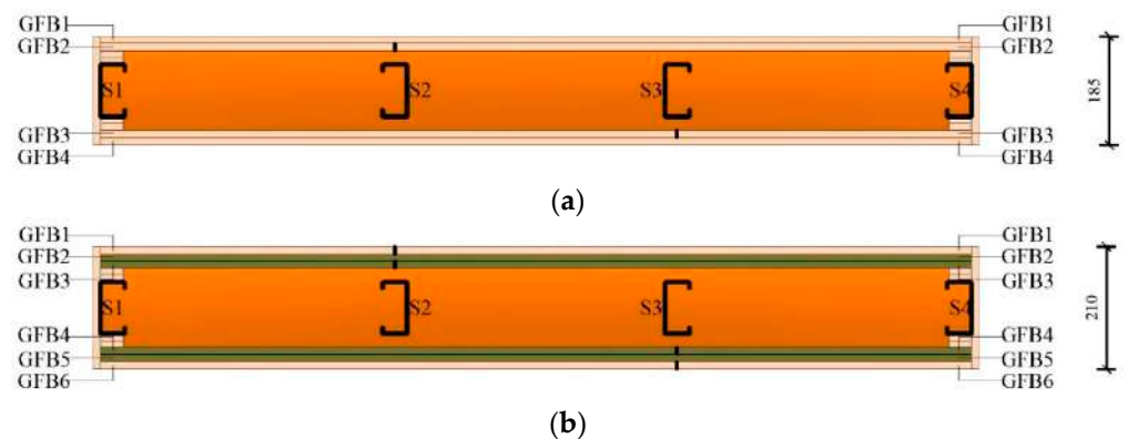
Figure 2. Wall configurations used in the fire tests: (a) Cross section of the double lined specimens (P1 and P2); (b) cross section of triple lined specimen (P3).
