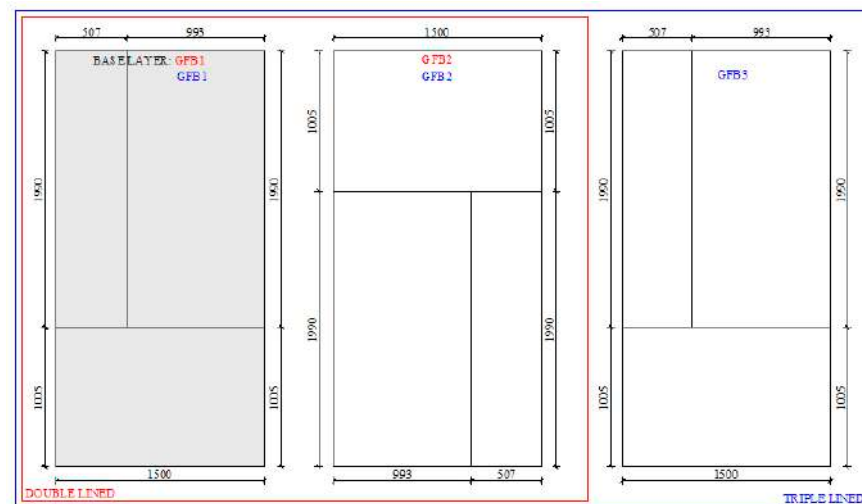
Figure 3. GFB wallboard lining configuration. The red box indicates the wallboard configuration for double-lined, while blue box for triple-lined LSF walls.
