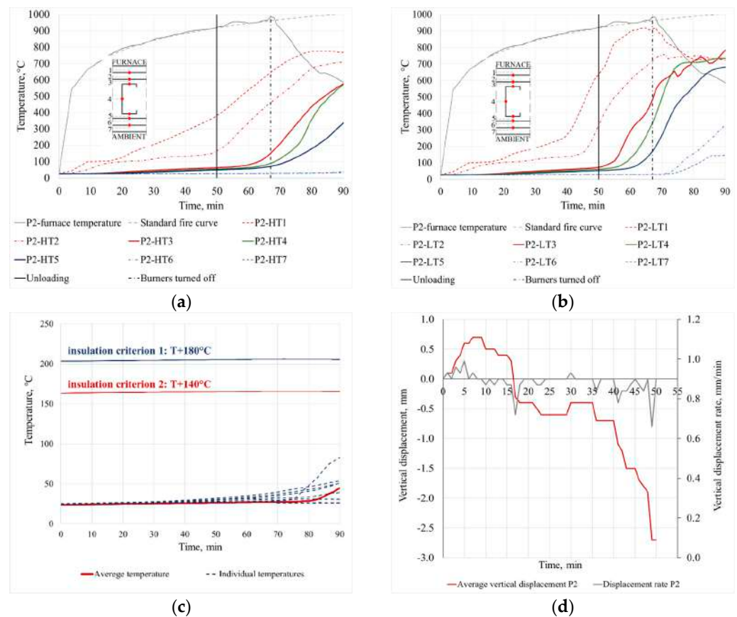
Figure 7. Fire test results for specimen P2: (a) average temperatures at high positions (HTs); (b) average temperatures at low positions (LTs); (c) temperatures recorded at the unexposed side of the specimen; (d) average vertical displacement and displacement rate.
