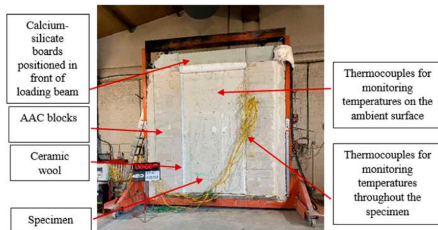
Figure 5. Specimen set-up in the testing furnace.
