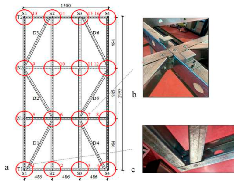
Figure 1. Layout of the LSF wall frame and characteristic connection details: (a) steel frame; (b) Z-shaped spacers near the node, (c) cut-out of the steel frame. Red circles numbered 1–16 indicate the 16 nodes formed in the steel frame.
