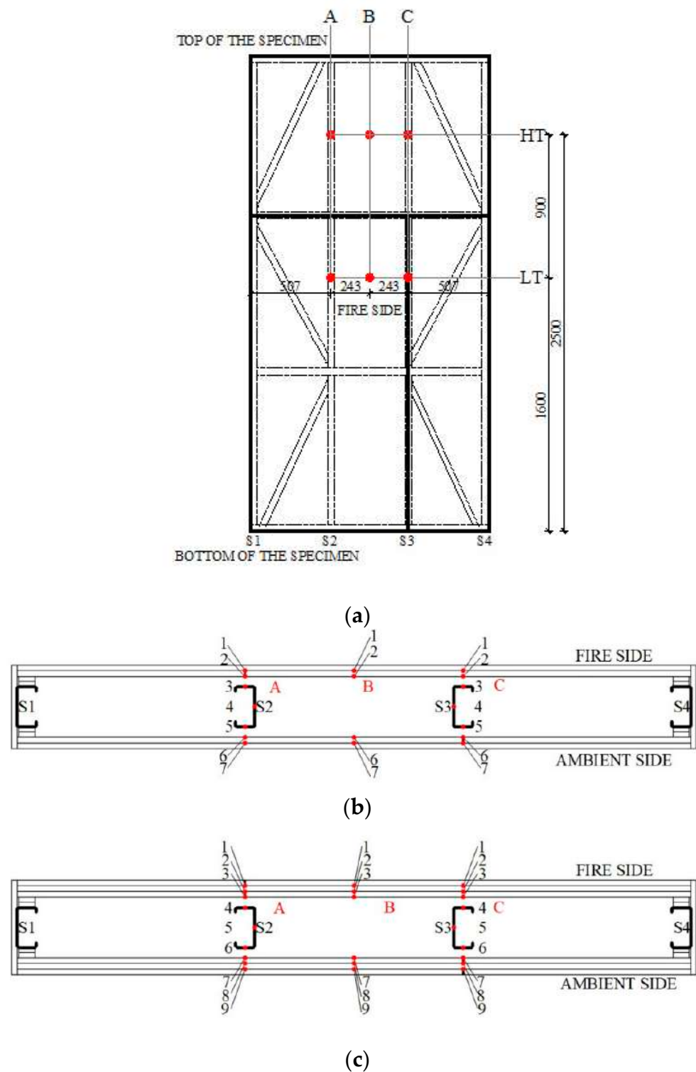
Figure 4. Thermocouple positions through the cross-sections of the specimens: (a) Front side of the test specimens; (b) cross-sections of specimens P1 and P2; (c) cross-section of specimen P3.
