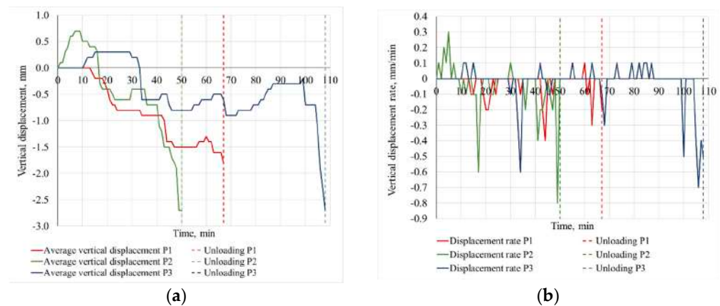
Figure 10. Comparison between the measured (a) displacements and (b) displacement rates.
