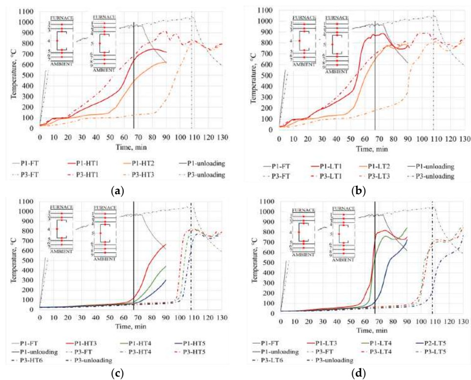
Figure 13. Time–temperature curves comparisons for specimen P1 and P3: (a) average time–temperature curves for higher positions (HTs); (b) average time–temperature curves for lower positions (LTs); (c) average time–temperature curves measured on the steel studs (HTs); (d) average time–temperature curves measured on steel studs (LTs).
