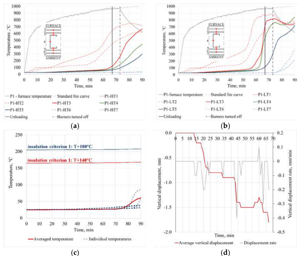
Figure 6. Fire test results for specimen P1: (a) average temperatures at high position (HTs); (b) average temperatures at low position (LTs); (c) temperature profiles at the unexposed side of the specimen; (d) average vertical displacement and displacement rate.
