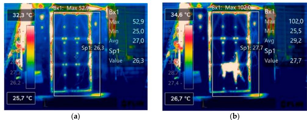
Figure 11. Thermograms for specimen P1: (a) in the 67th minute; (b) in the 76th minute.
