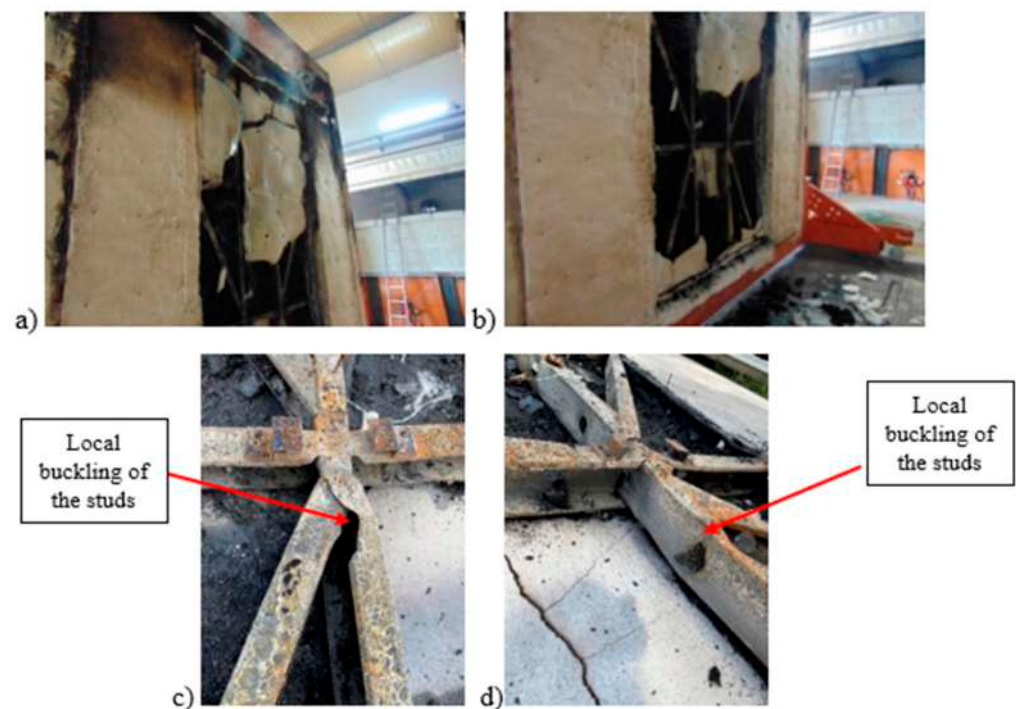
Figure 9. Post test observations for specimen P2: (a) exposed side of upper part of test specimen; (b) exposed side of lower part of test specimen; (c) node 6; (d) node 7.
