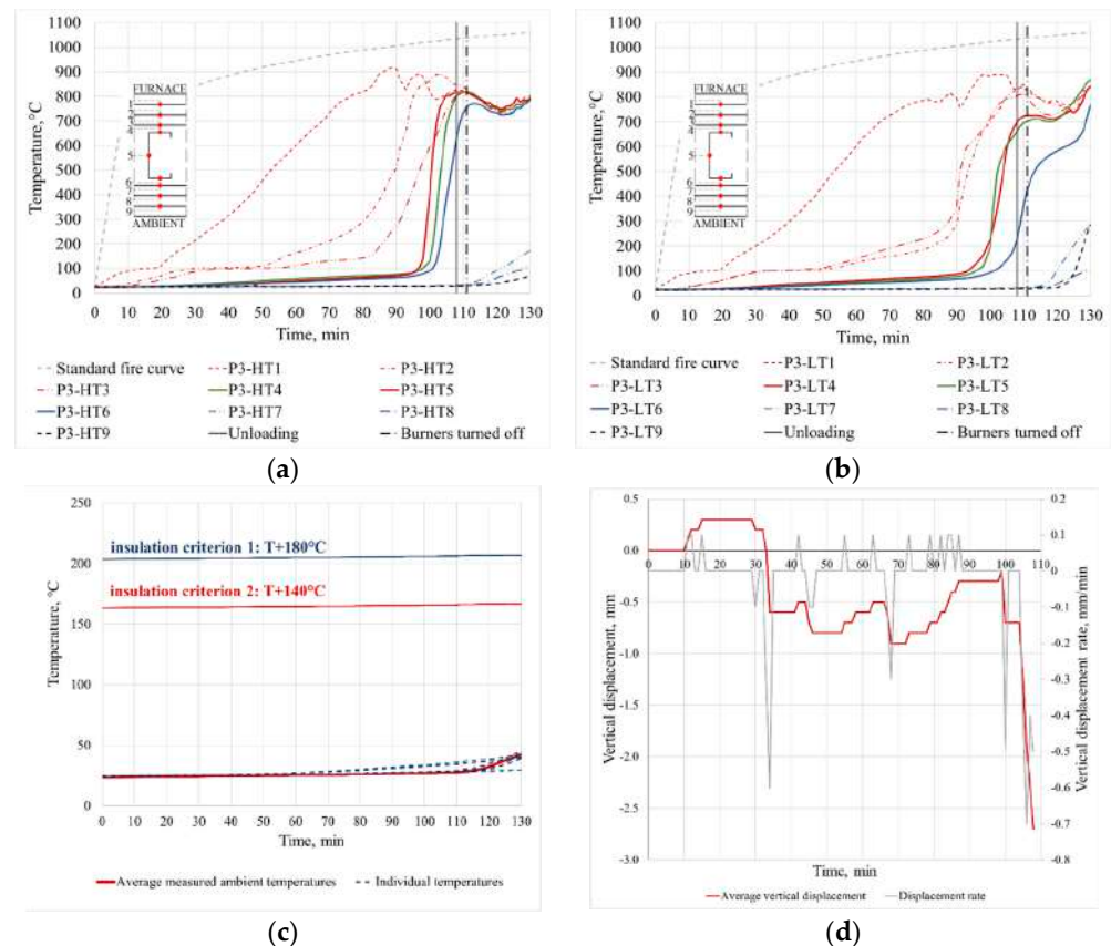
Figure 8. Fire test results for specimen P3: (a) average temperatures at high positions (HTs), (b) average temperatures at low positions (LTs); (c) temperatures recorded at the unexposed side of the specimen; (d) average vertical displacement and displacement rate.
